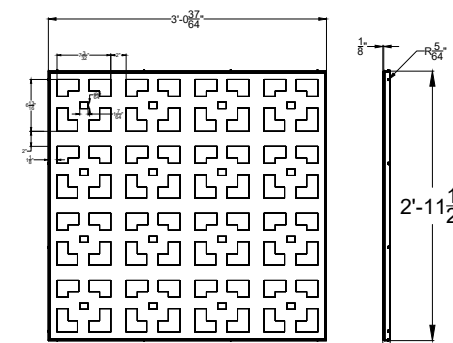
FRONT SIDE PANEL DETAILS (GARDEN PARTY)
