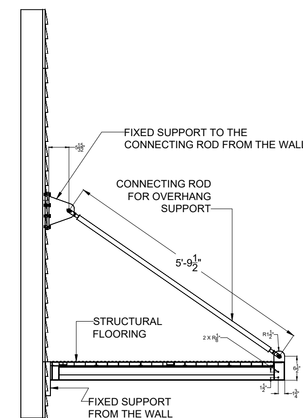
STRUCTURAL FLOORING WITH CONNECTING ROD
