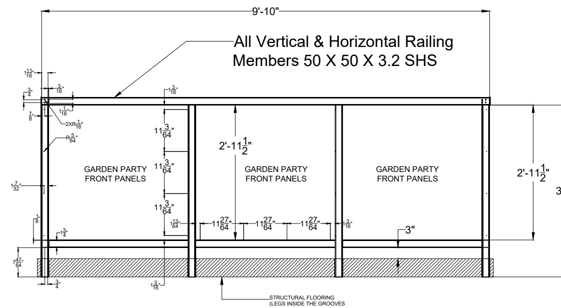
FRONT VIEW (WITHOUT PANEL )
