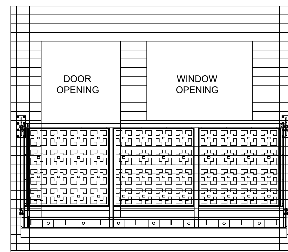
FRONT VIEW (WITH BACK SIDE WALL)
