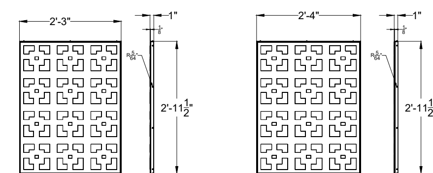
SIDE PANEL 2 DETAILS
